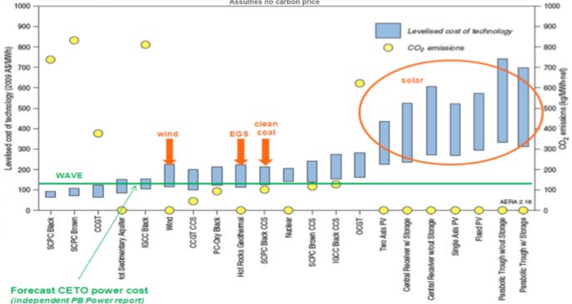
Independent EPRI technology status data, 2010
